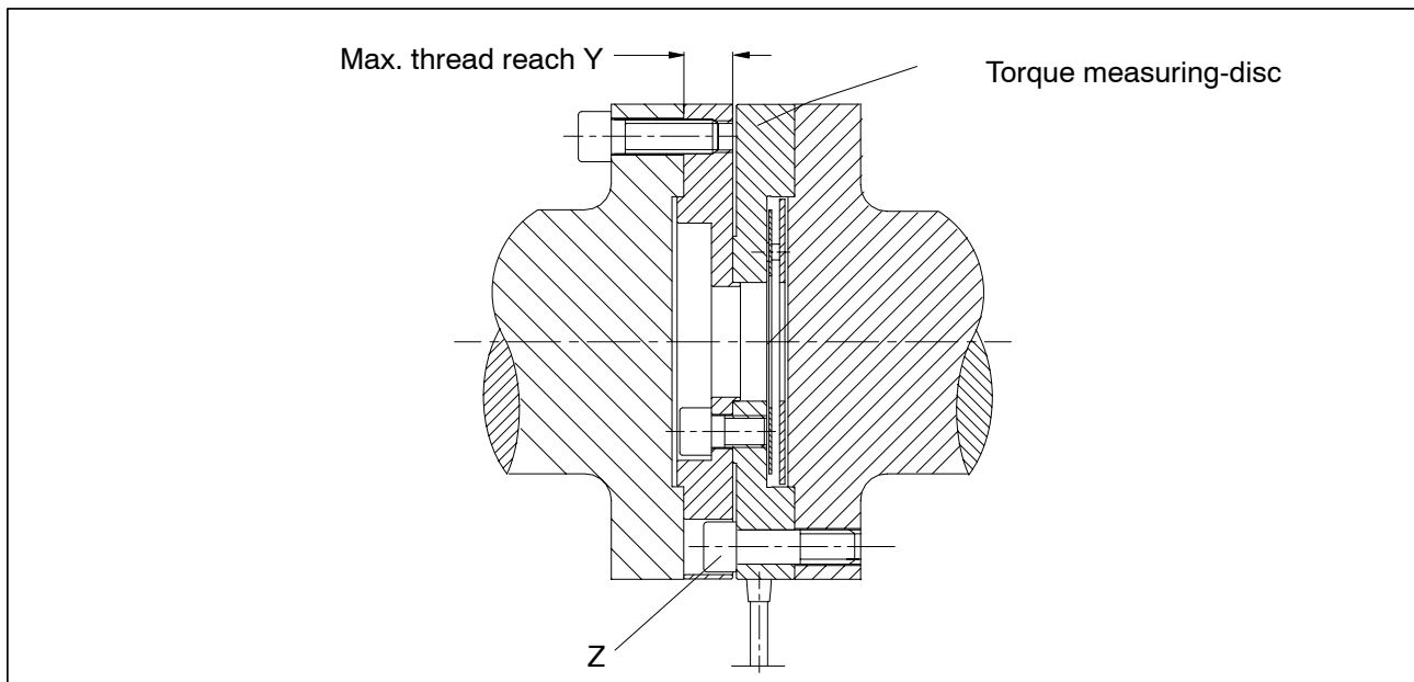
Fig.4.4: Installation example
